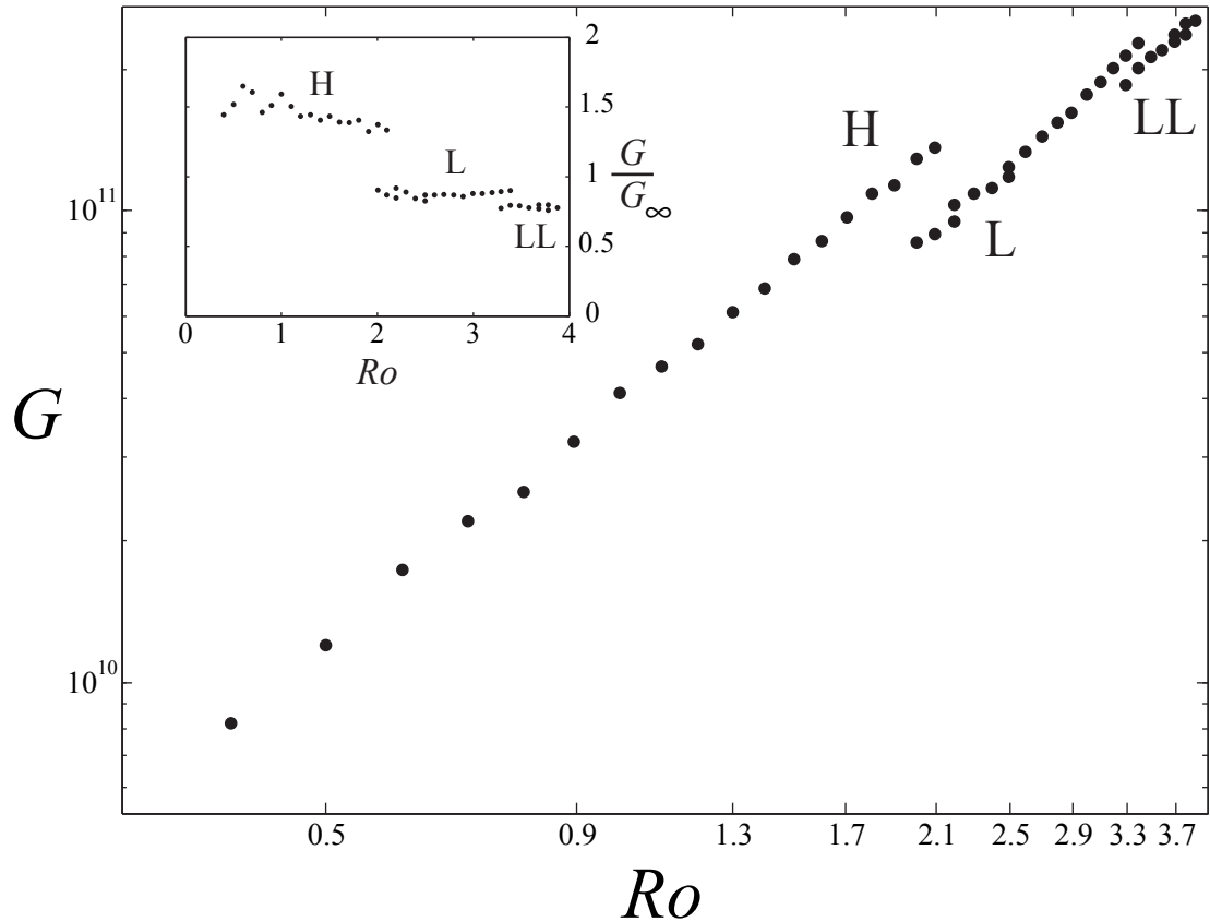
Fig. 4.14: Torque as a function of Rossby, E = 1.6 \times 10^{-7} , with compensated torque inset. Where bimodal torque distributions are noted, the torque is split into two branches corresponding to the two modes. Overlapping regions are associated with intermittent transitions between the two turbulent flow states adjacent to the switching region.
