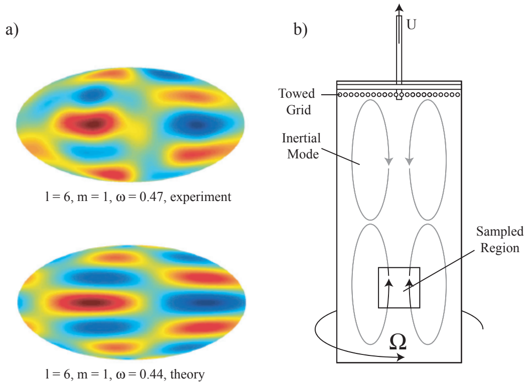
Fig. 1.6: Inertial modes in turbulent flows result in global flow correlations and inhomogeneity. At (a), a Mollweide projection of the external induced magnetic field (top) in rapidly rotating turbulent spherical Couette flow with weak axial applied field is compared with the induction predicted for that expected from a single matching inertial mode (bottom). The experimental measurements of Kelley et al. [14] show a strong signature of the identified mode along with additional fluctuating induction. At (b), a schematic depiction of the results of Bewley et al. [60]. Inertial modes excited by a towed grid in rotating, decaying turbulence result in oscillatory flows at large scales with respect to the measurement volume. Several inertial modes are observed as the turbulence decays. Excerpted images from Kelley et al. , 2007 [14] reproduced here with permission from Taylor and Francis Group, Ltd.
